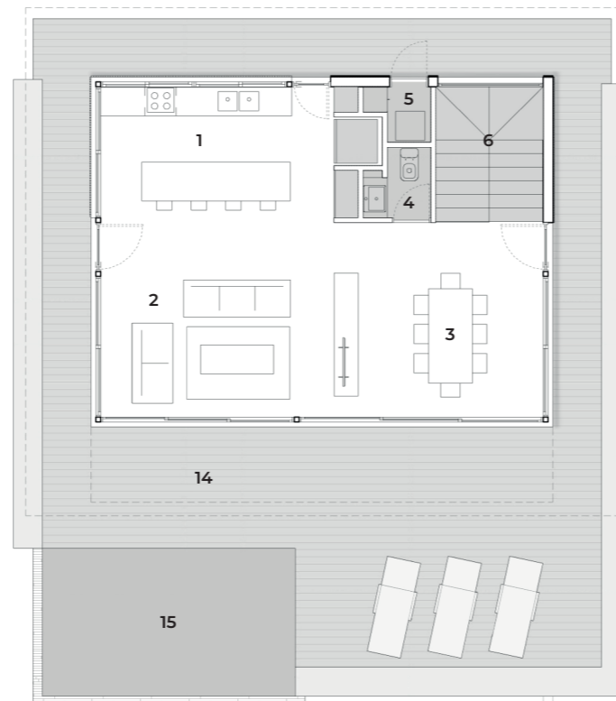
Floor Plan L00
