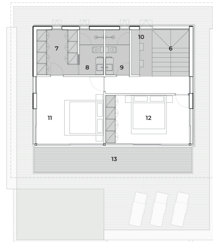
Floor Plan L01
